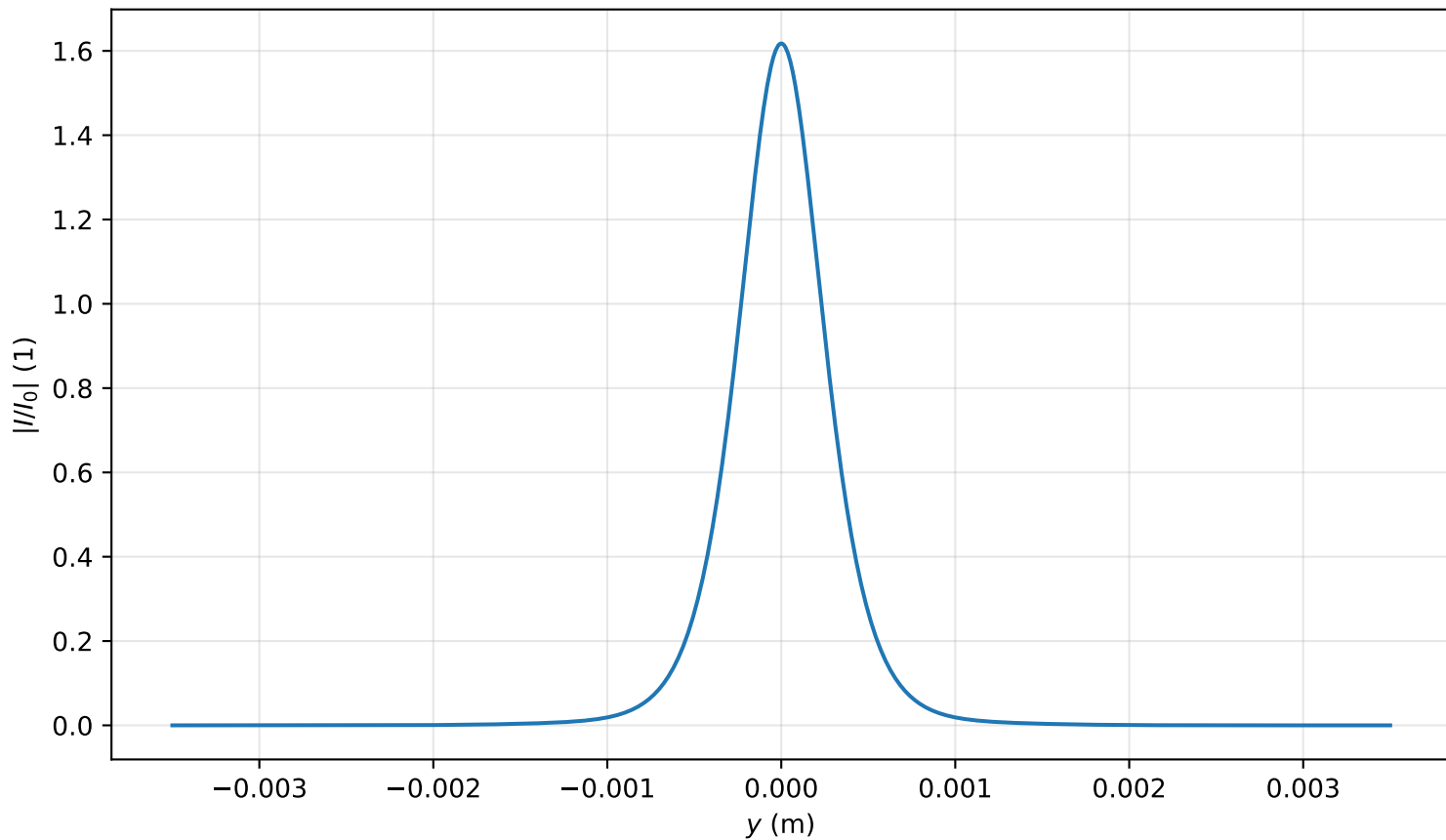
Intensity profile I(x=0, y, z=2.548)/I_0 , P_{in}=0.9P_{cr} , artificial time
